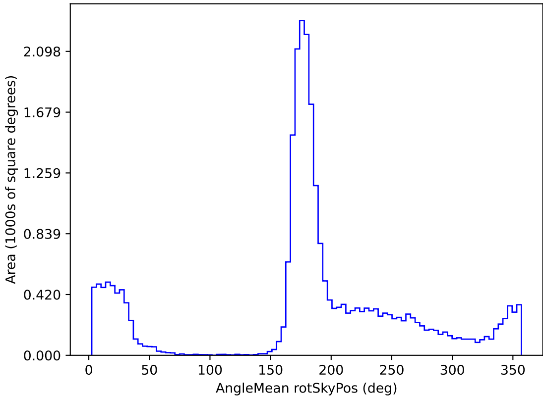
roll_pause_mjdp120_v3.4_10yrs All sky r band: AngleMean rotSkyPos
