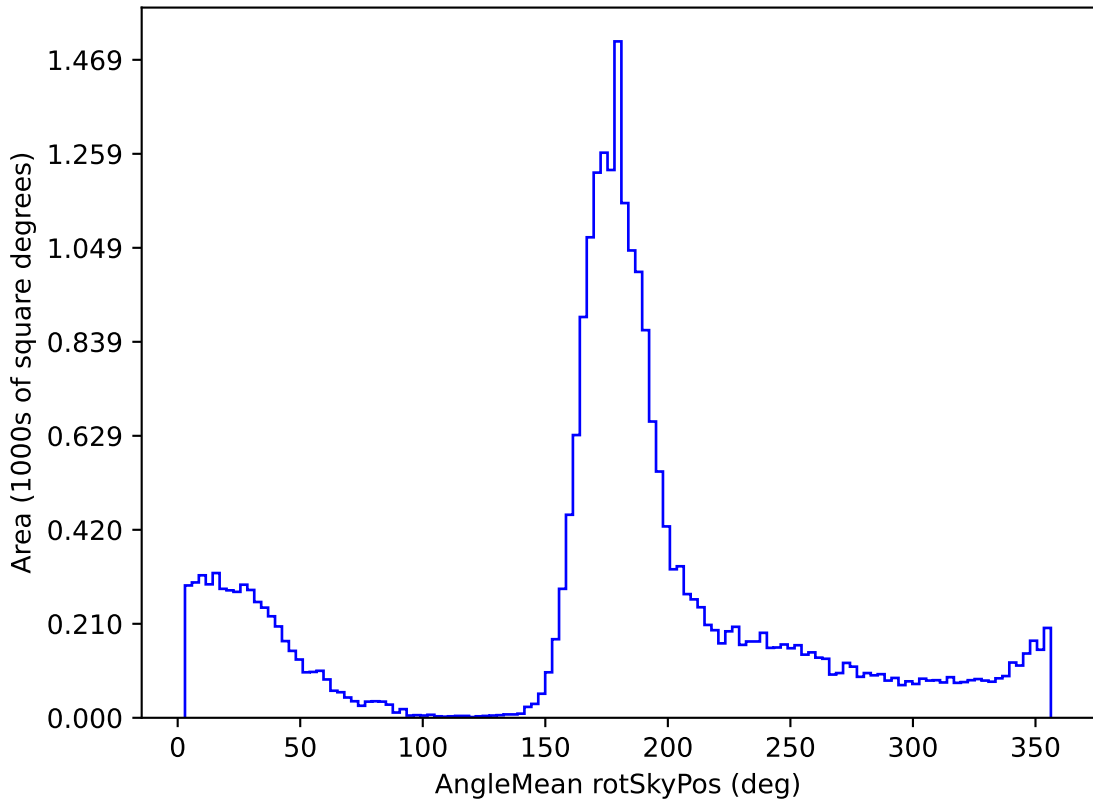
roll_pause_mjdp120_v3.4_10yrs All sky g band: AngleMean rotSkyPos
