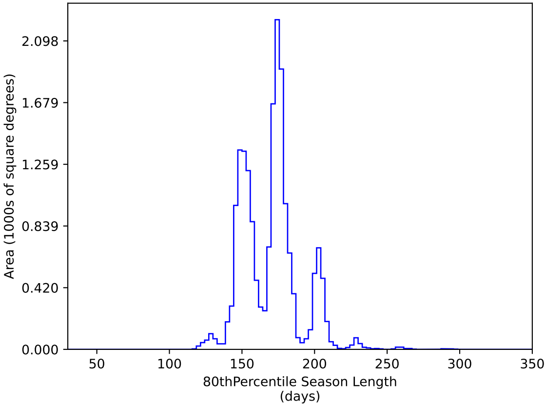
roll_pause_mjdp120_v3.4_10yrs WFD y band: 80thPercentile Season Length
