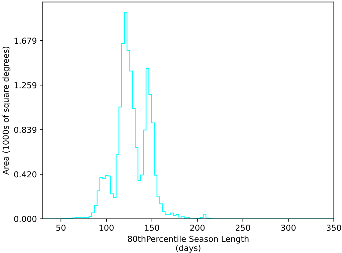
roll_pause_mjdp120_v3.4_10yrs WFD u band: 80thPercentile Season Length
