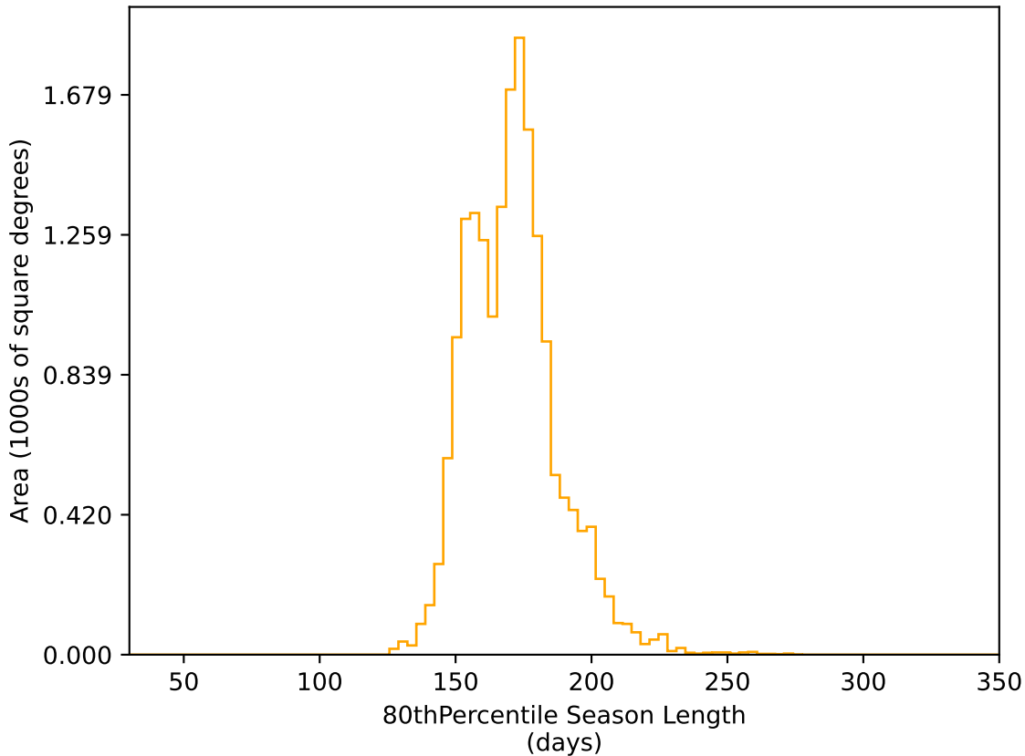
roll_pause_mjdp120_v3.4_10yrs WFD r band: 80thPercentile Season Length
