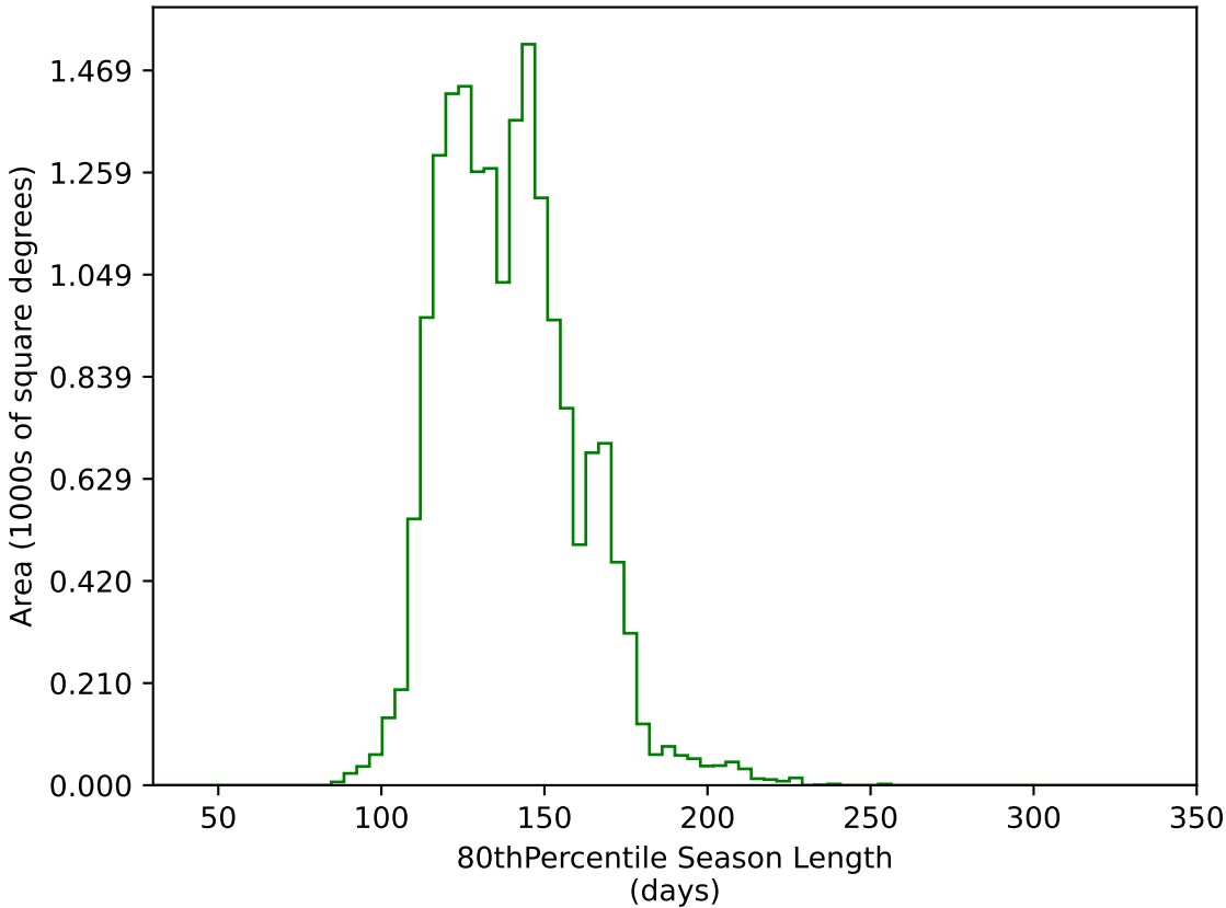
roll_pause_mjdp120_v3.4_10yrs WFD g band: 80thPercentile Season Length
