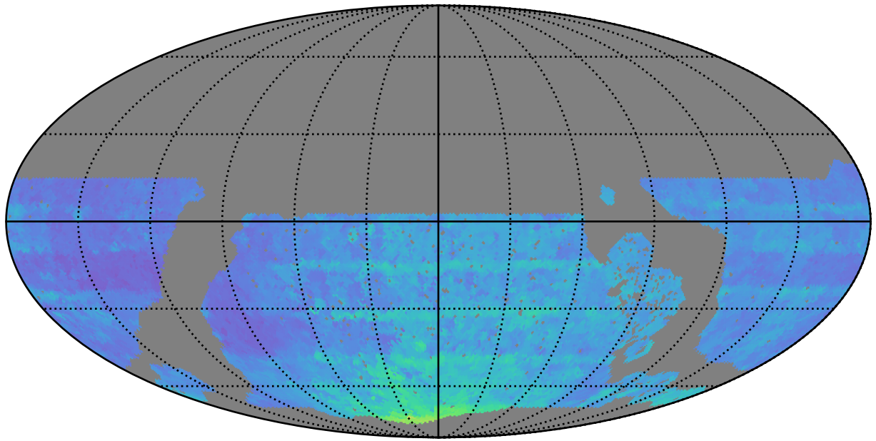
roll_pause_mjdp120_v3.4_10yrs WFD all bands: 80thPercentile Season Length
