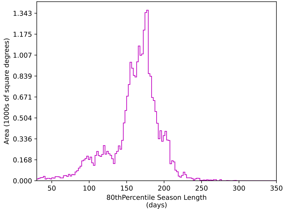
roll_pause_mjdp120_v3.4_10yrs All sky z band: 80thPercentile Season Length
