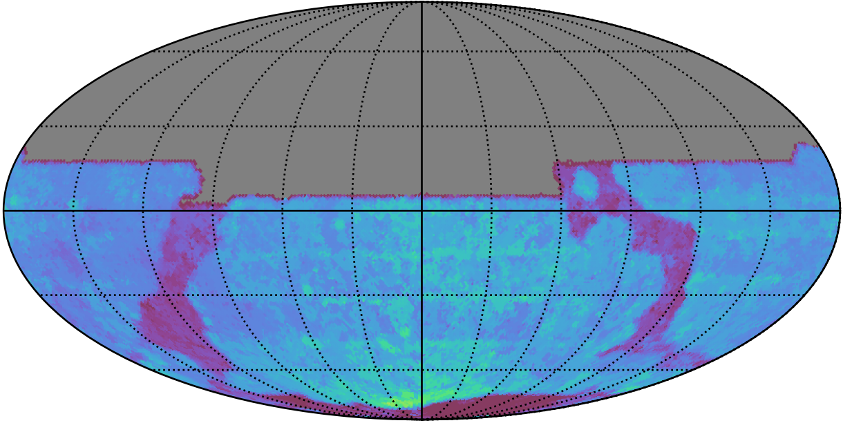
roll_pause_mjdp120_v3.4_10yrs All sky y band: 80thPercentile Season Length
