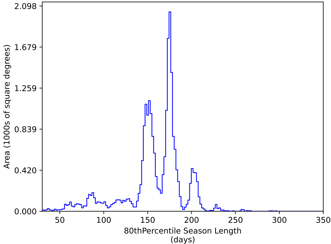
roll_pause_mjdp120_v3.4_10yrs All sky y band: 80thPercentile Season Length
