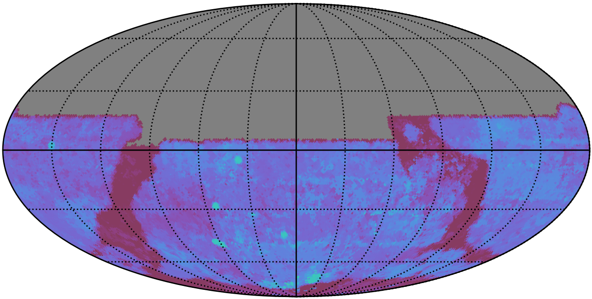
roll_pause_mjdp120_v3.4_10yrs All sky u band: 80thPercentile Season Length
