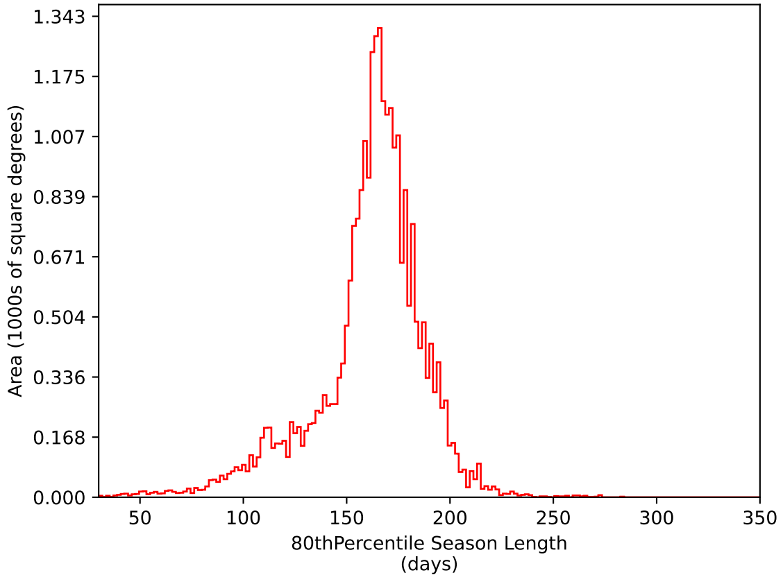
roll_pause_mjdp120_v3.4_10yrs All sky i band: 80thPercentile Season Length
