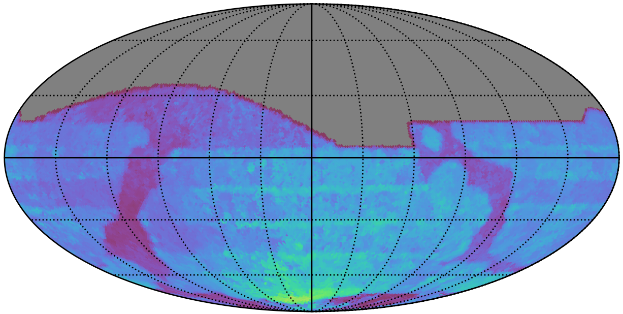
roll_pause_mjdp120_v3.4_10yrs All sky all bands: 80thPercentile Season Length
