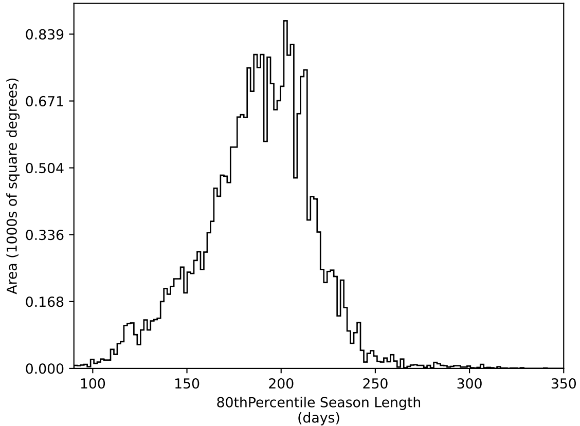
roll_pause_mjdp120_v3.4_10yrs All sky all bands: 80thPercentile Season Length
