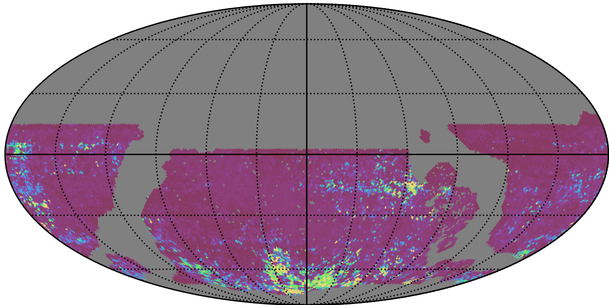
roll_pause_mjdp120_v3.4_10yrs WFD z band: 75th Percentile Intranight Timespan
