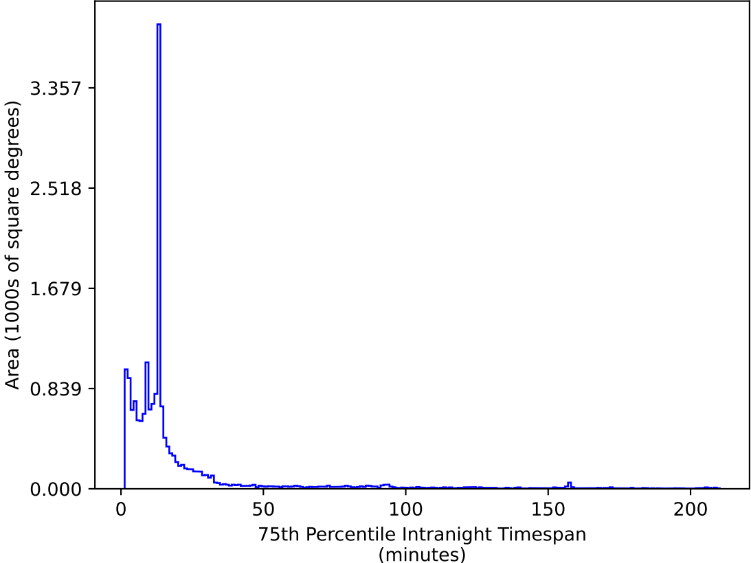
roll_pause_mjdp120_v3.4_10yrs WFD z band: 75th Percentile Intranight Timespan
