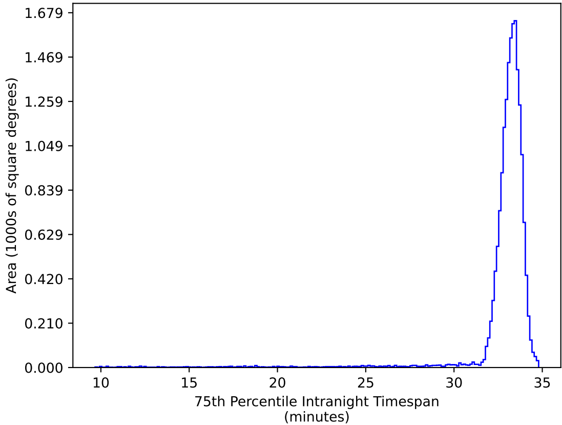
roll_pause_mjdp120_v3.4_10yrs WFD ug bands: 75th Percentile Intranight Timespan
