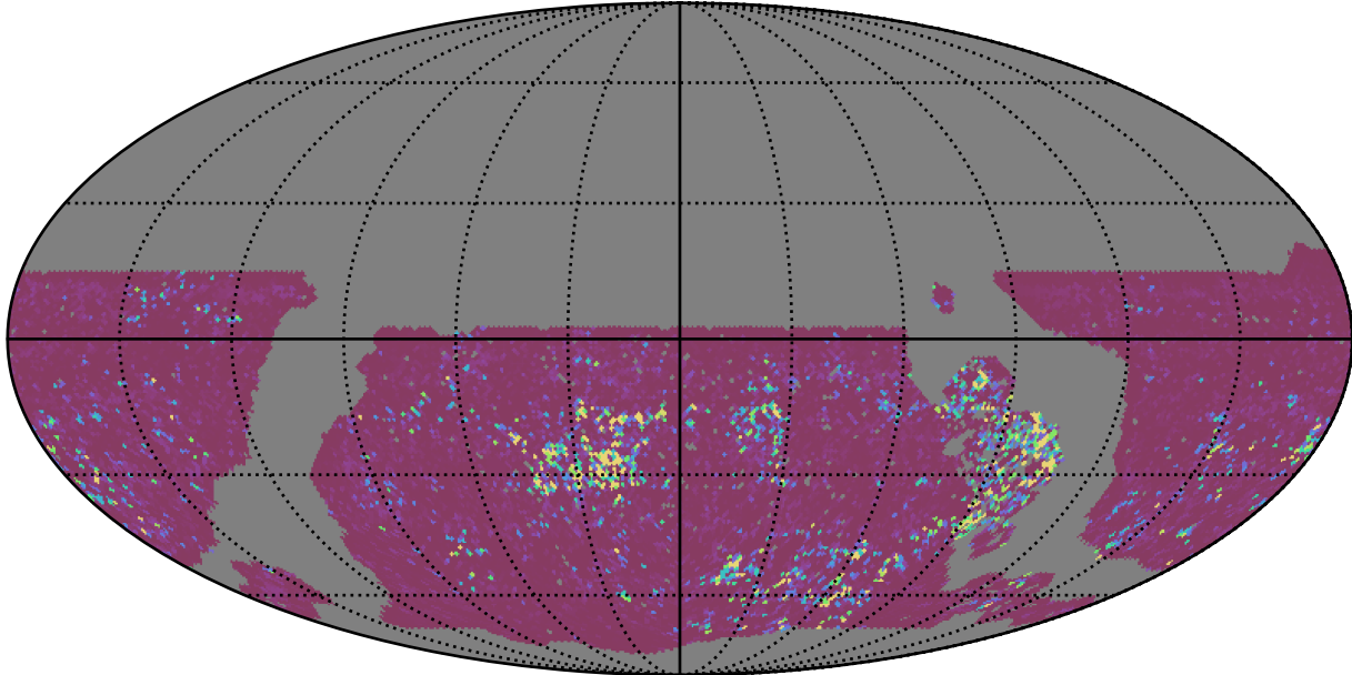
roll_pause_mjdp120_v3.4_10yrs WFD u band: 75th Percentile Intranight Timespan
