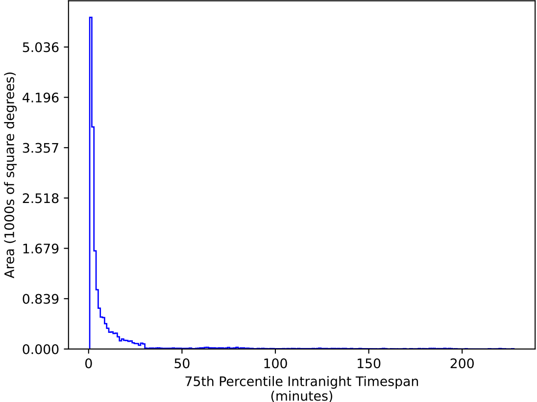
roll_pause_mjdp120_v3.4_10yrs WFD u band: 75th Percentile Intranight Timespan
