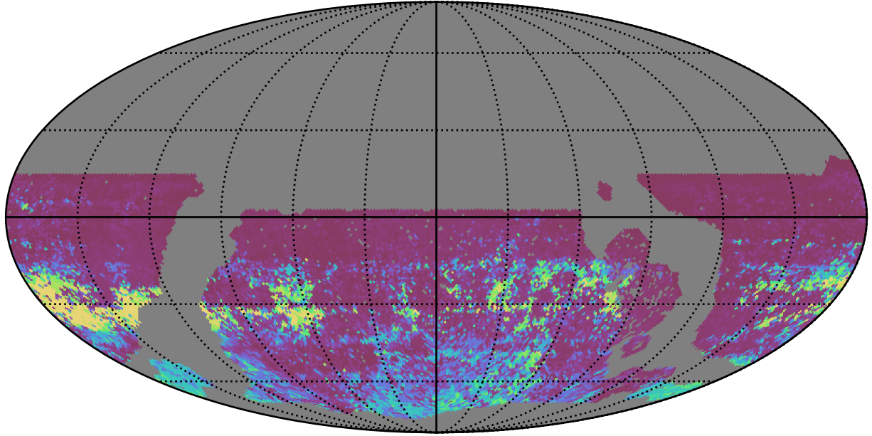
roll_pause_mjdp120_v3.4_10yrs WFD r band: 75th Percentile Intranight Timespan
