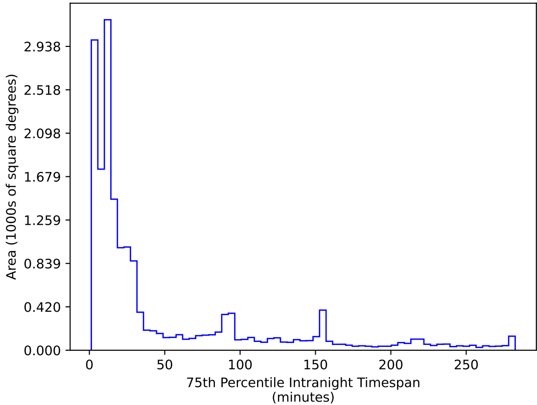
roll_pause_mjdp120_v3.4_10yrs WFD r band: 75th Percentile Intranight Timespan
