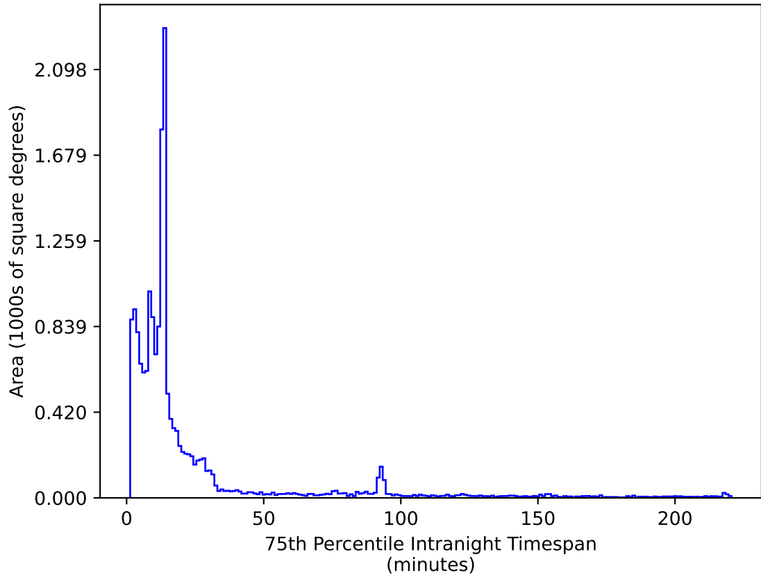
roll_pause_mjdp120_v3.4_10yrs WFD i band: 75th Percentile Intranight Timespan
