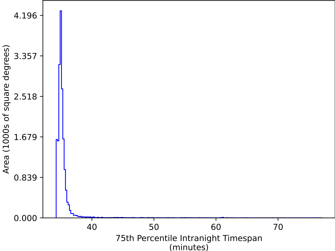
roll_pause_mjdp120_v3.4_10yrs WFD gr bands: 75th Percentile Intranight Timespan
