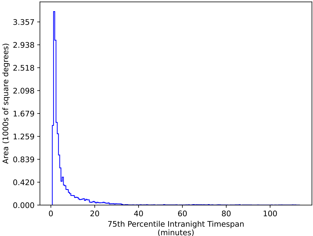
roll_pause_mjdp120_v3.4_10yrs WFD g band: 75th Percentile Intranight Timespan
