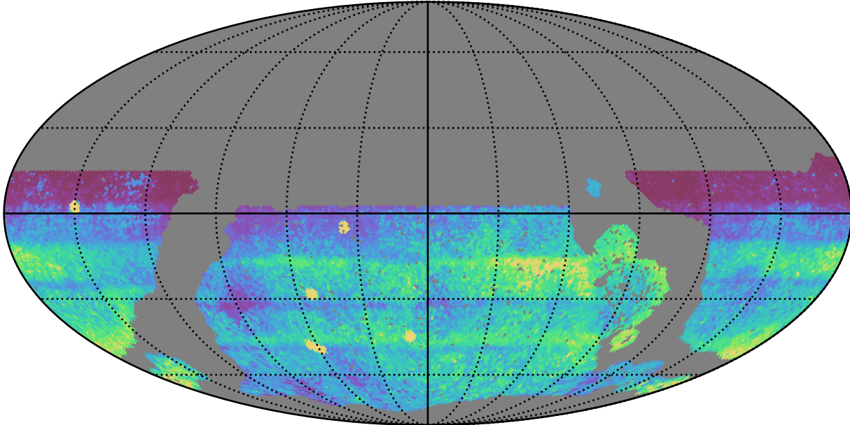
roll_pause_mjdp120_v3.4_10yrs WFD all bands: 75th Percentile Intranight Timespan
