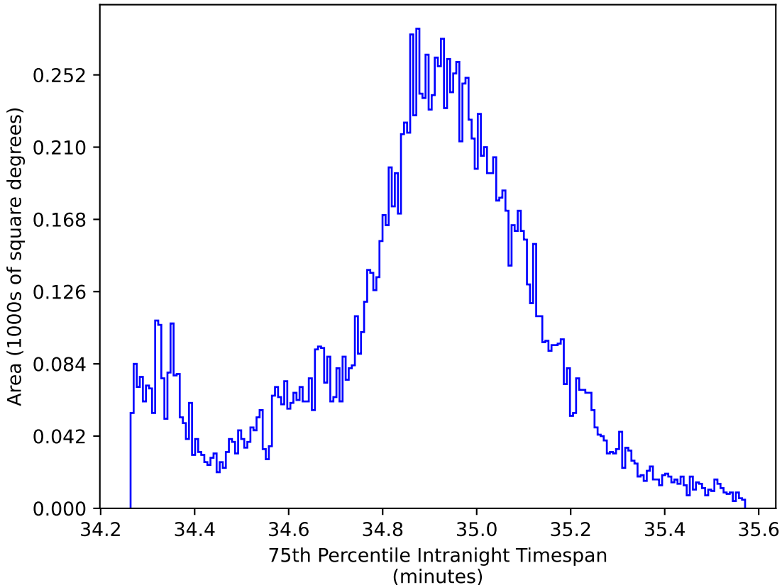
roll_pause_mjdp120_v3.4_10yrs WFD all bands: 75th Percentile Intranight Timespan
