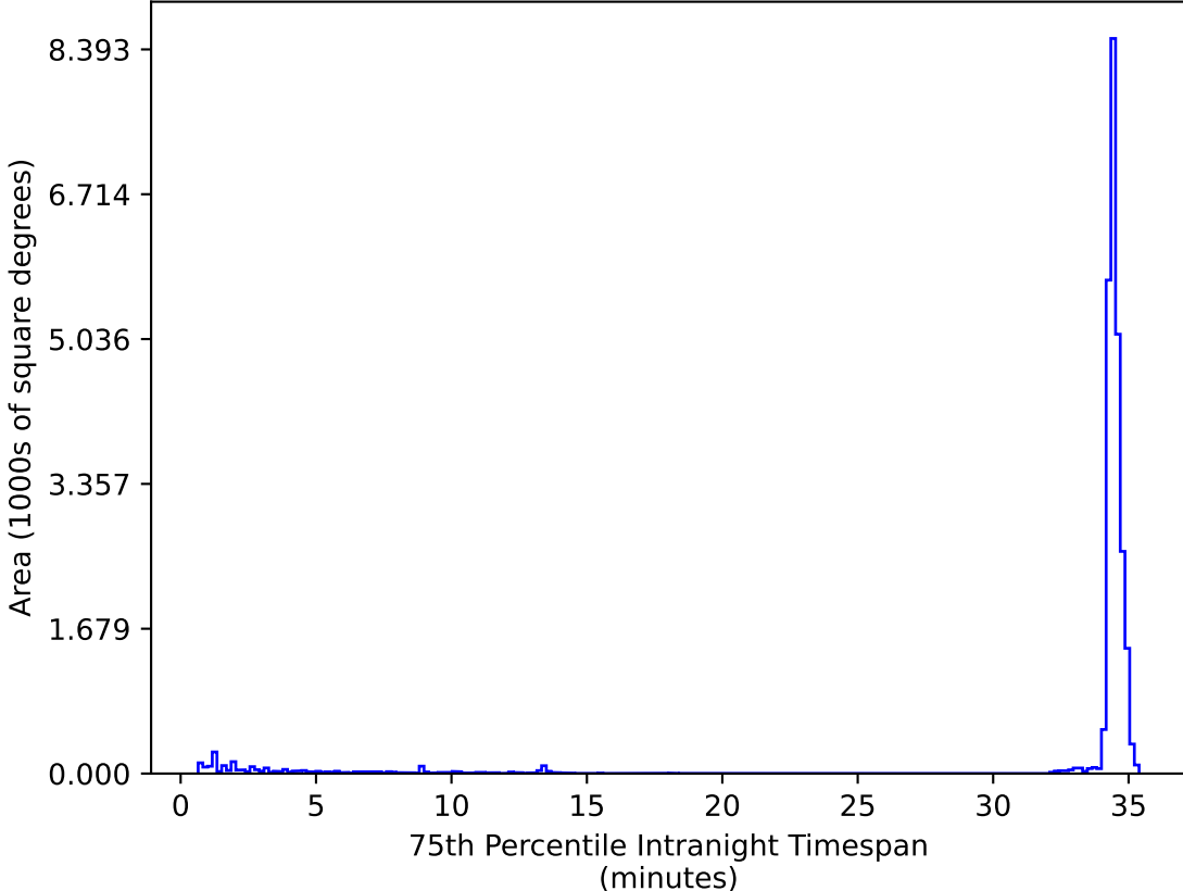
roll_pause_mjdp120_v3.4_10yrs All sky zy bands: 75th Percentile Intranight Timespan
