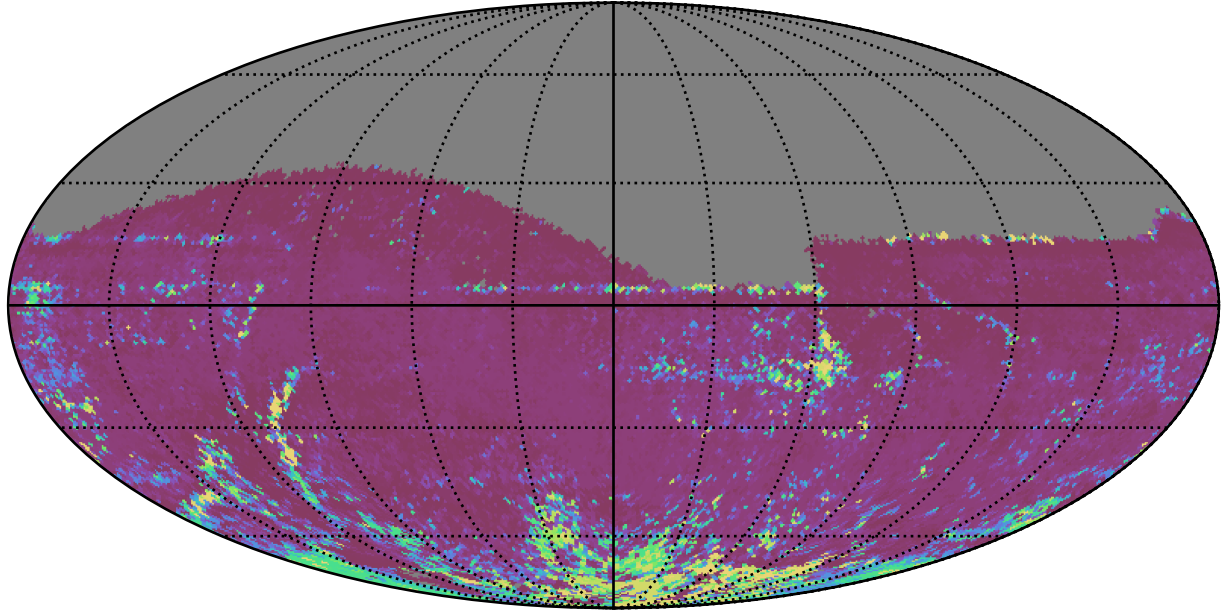
roll_pause_mjdp120_v3.4_10yrs All sky z band: 75th Percentile Intranight Timespan
