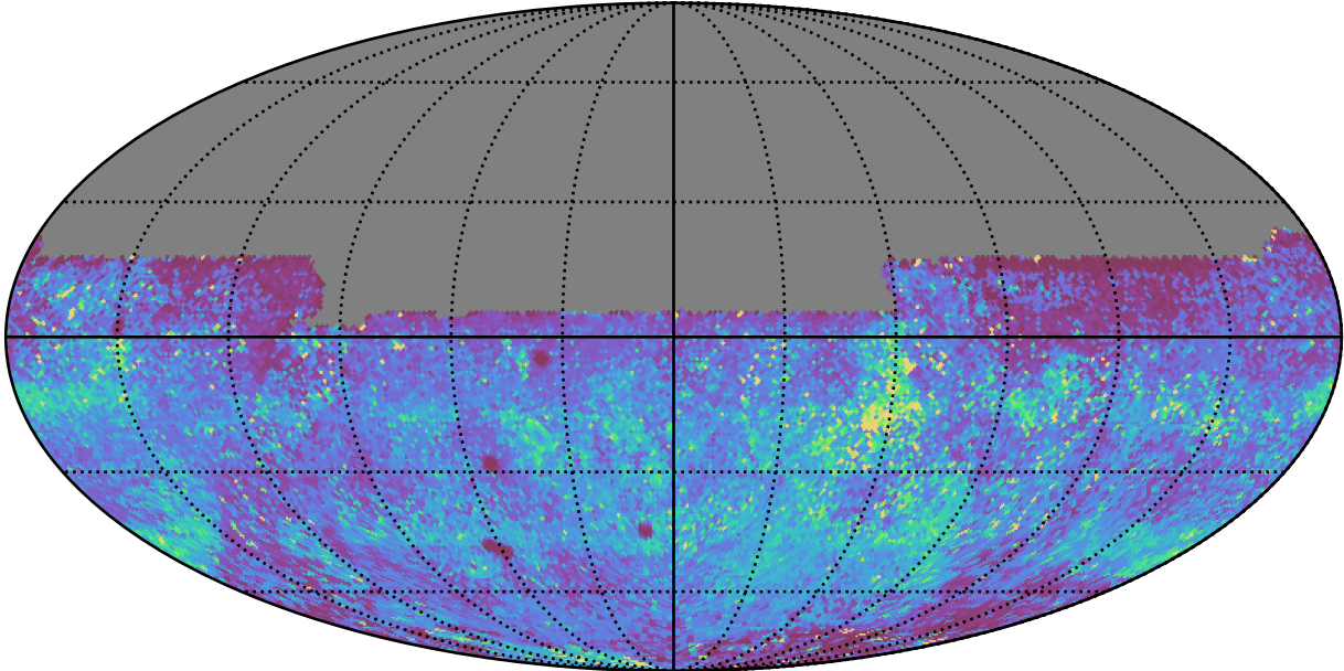
roll_pause_mjdp120_v3.4_10yrs All sky y band: 75th Percentile Intranight Timespan
