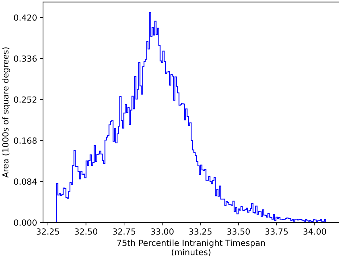
roll_pause_mjdp120_v3.4_10yrs All sky y band: 75th Percentile Intranight Timespan
