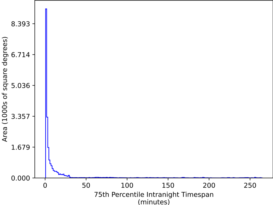
roll_pause_mjdp120_v3.4_10yrs All sky u band: 75th Percentile Intranight Timespan
