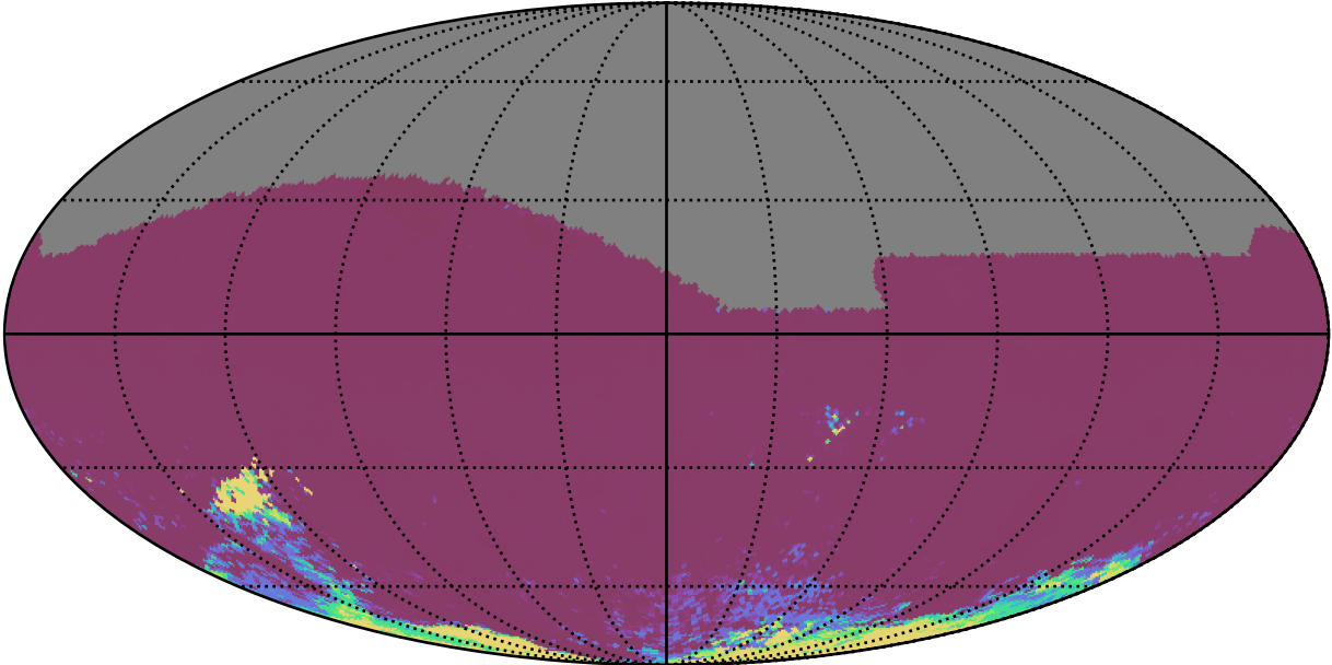
roll_pause_mjdp120_v3.4_10yrs All sky ri bands: 75th Percentile Intranight Timespan
