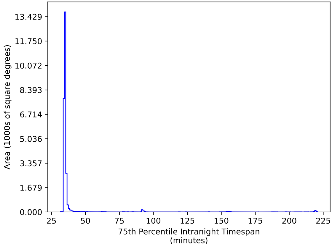
roll_pause_mjdp120_v3.4_10yrs All sky ri bands: 75th Percentile Intranight Timespan
