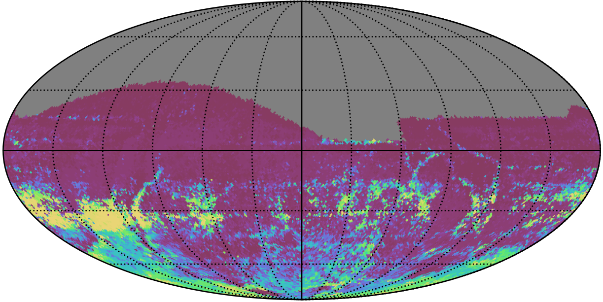
roll_pause_mjdp120_v3.4_10yrs All sky r band: 75th Percentile Intranight Timespan
