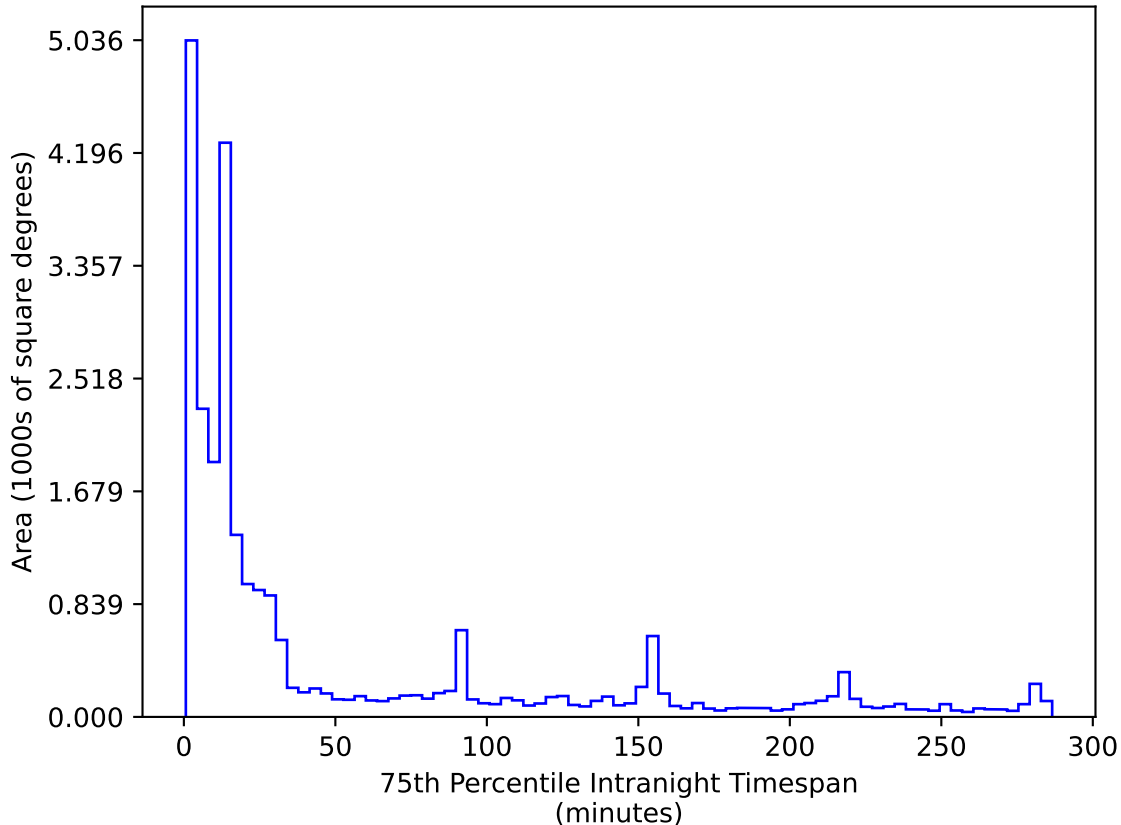
roll_pause_mjdp120_v3.4_10yrs All sky r band: 75th Percentile Intranight Timespan
