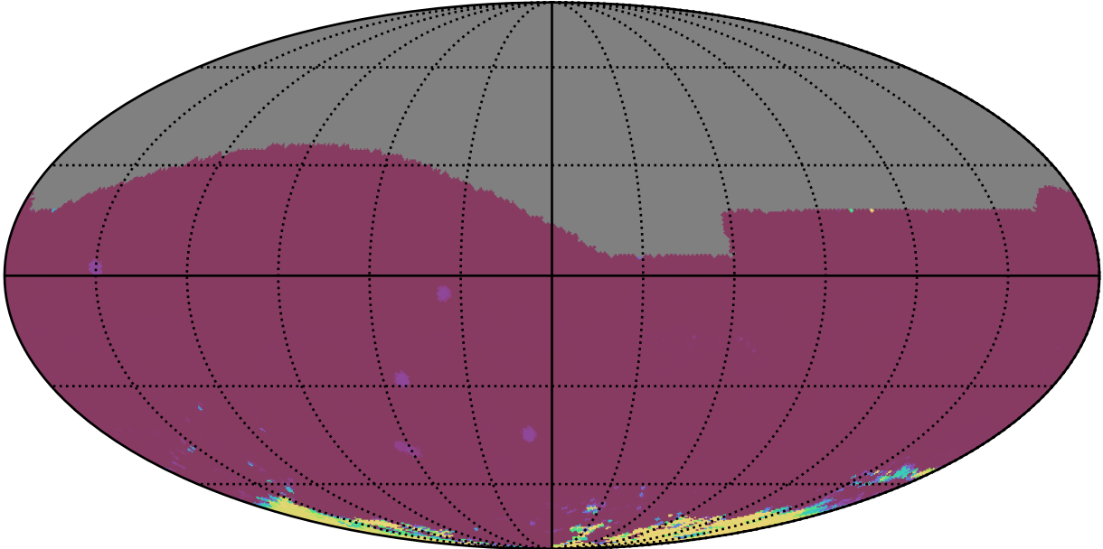
roll_pause_mjdp120_v3.4_10yrs All sky iz bands: 75th Percentile Intranight Timespan
