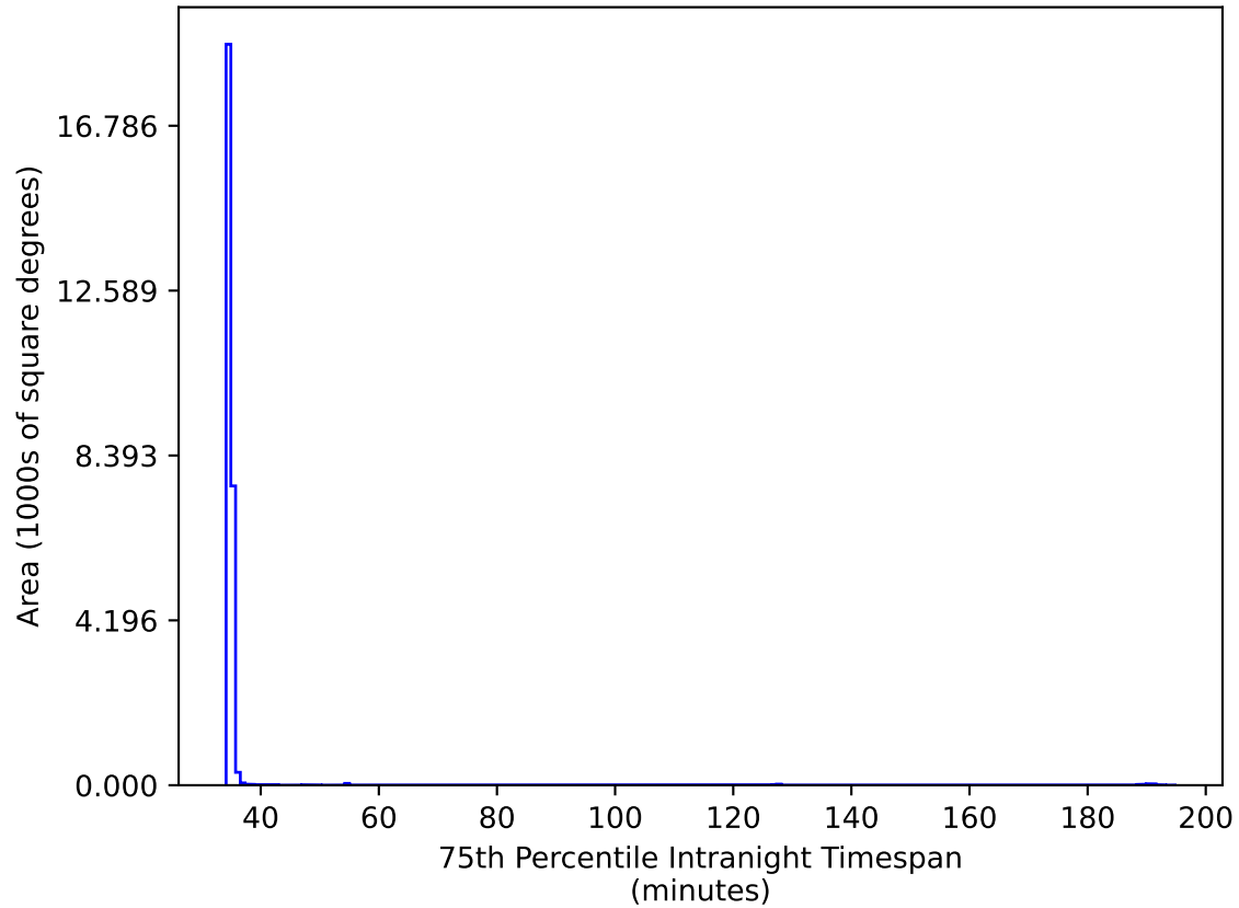
roll_pause_mjdp120_v3.4_10yrs All sky iz bands: 75th Percentile Intranight Timespan
