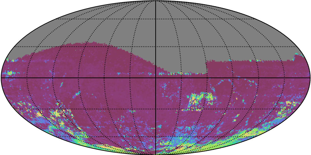
roll_pause_mjdp120_v3.4_10yrs All sky i band: 75th Percentile Intranight Timespan
