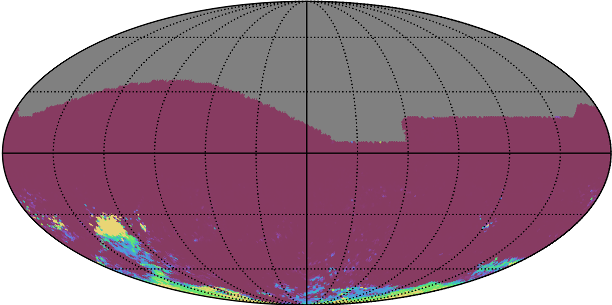
roll_pause_mjdp120_v3.4_10yrs All sky gr bands: 75th Percentile Intranight Timespan
