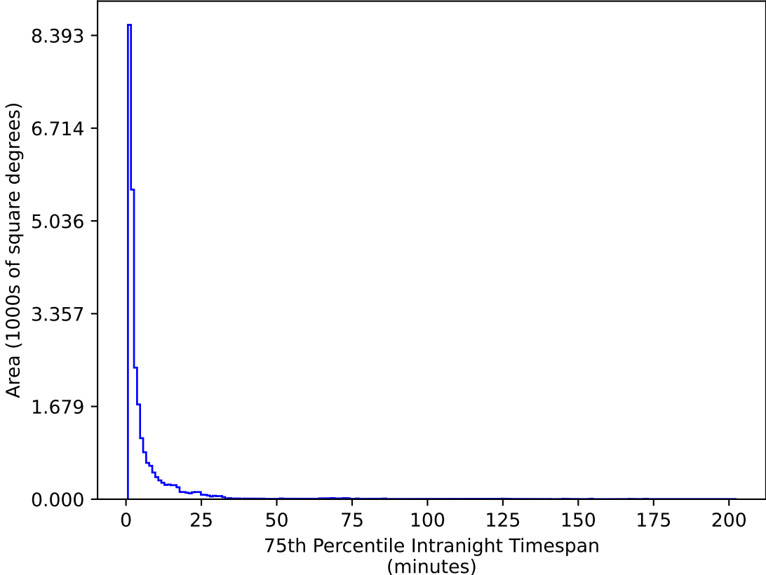
roll_pause_mjdp120_v3.4_10yrs All sky g band: 75th Percentile Intranight Timespan
