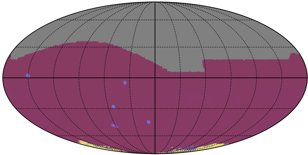
roll_pause_mjdp120_v3.4_10yrs All sky all bands: 75th Percentile Intranight Timespan
