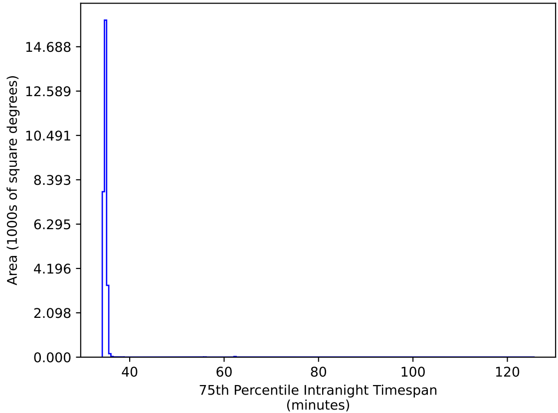
roll_pause_mjdp120_v3.4_10yrs All sky all bands: 75th Percentile Intranight Timespan
