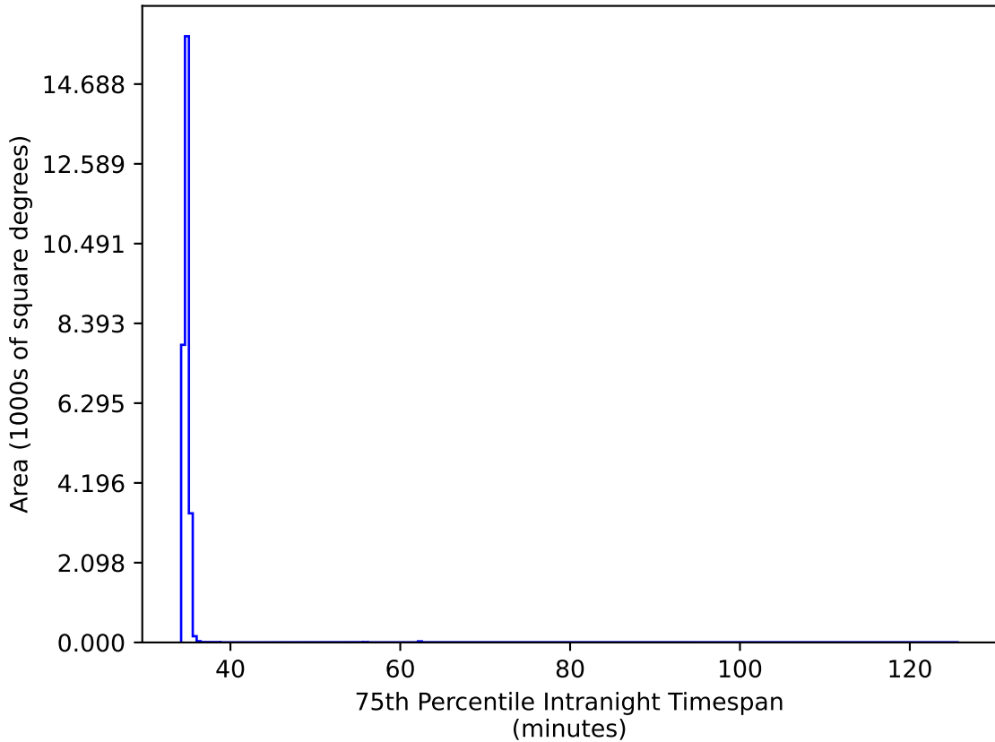
roll_pause_mjdp120_v3.4_10yrs All sky: 75th Percentile Intranight Timespan
