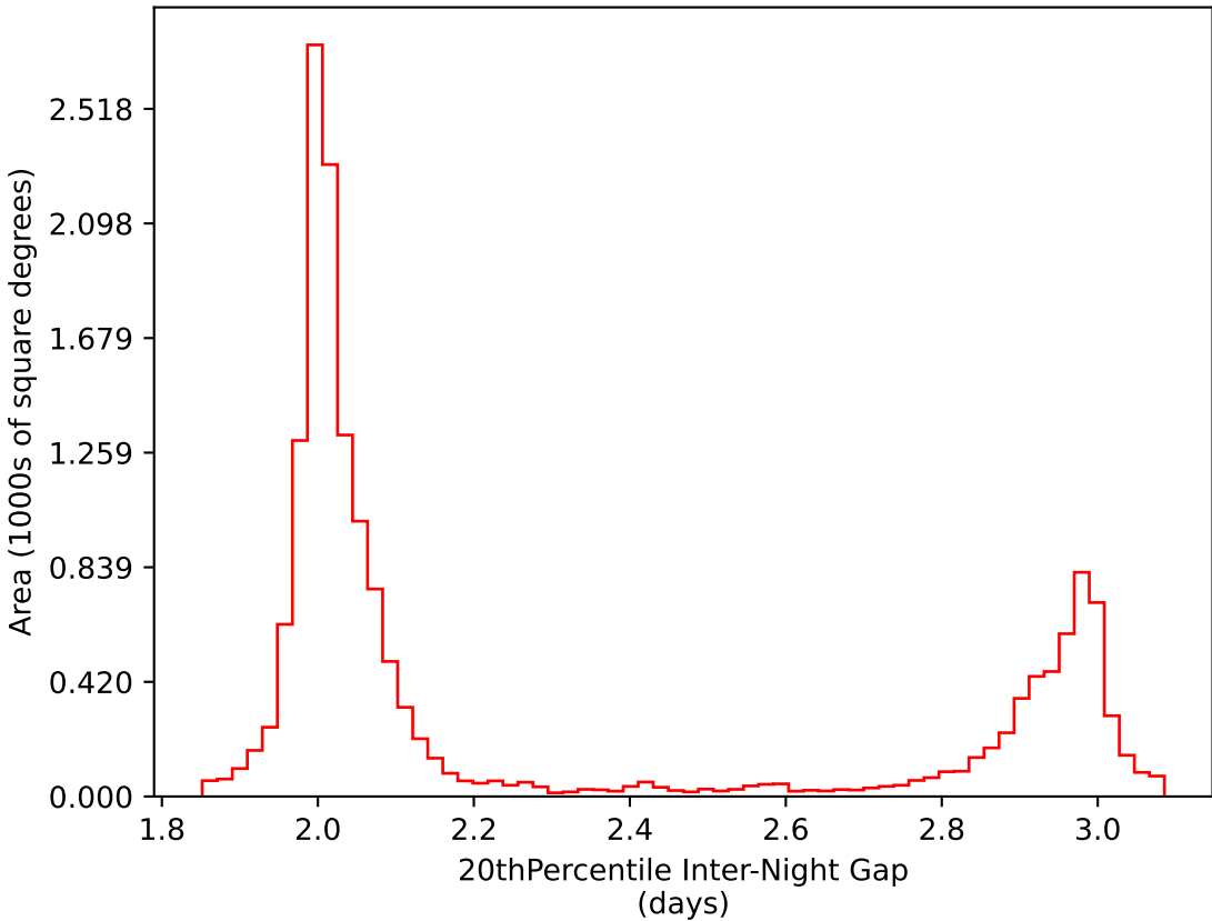
roll_pause_mjdp120_v3.4_10yrs WFD i band: 20thPercentile Inter-Night Gap
