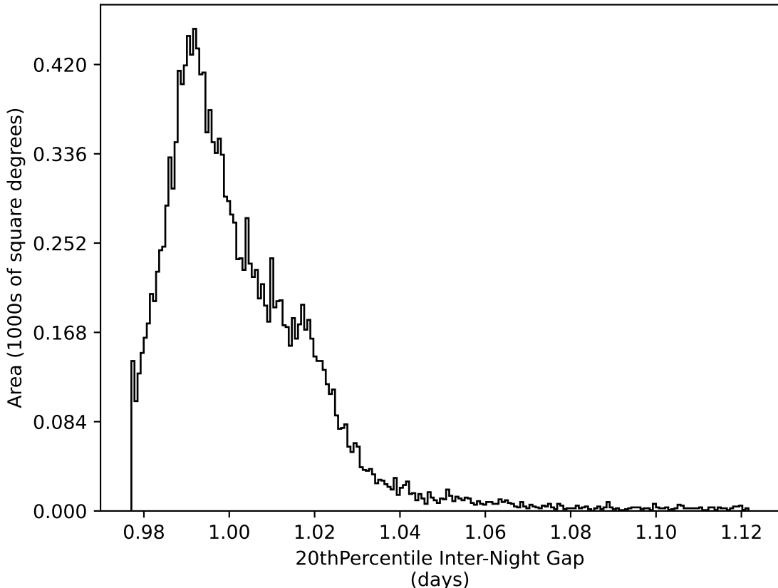
roll_pause_mjdp120_v3.4_10yrs WFD all bands: 20thPercentile Inter-Night Gap
