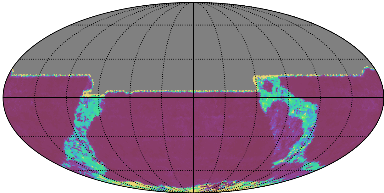
roll_pause_mjdp120_v3.4_10yrs All sky y band: 20thPercentile Inter-Night Gap
