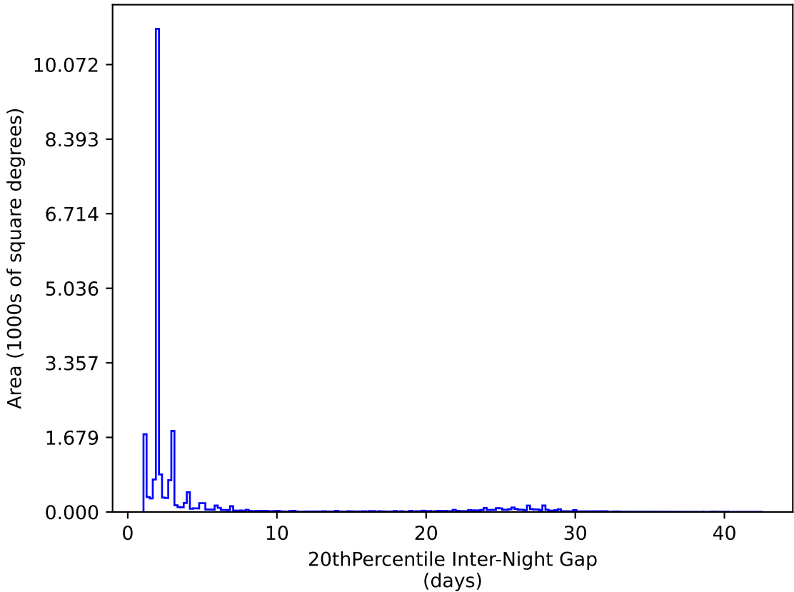
roll_pause_mjdp120_v3.4_10yrs All sky y band: 20thPercentile Inter-Night Gap
