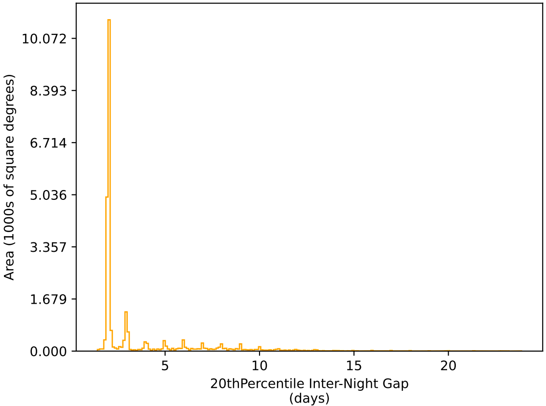
roll_pause_mjdp120_v3.4_10yrs All sky r band: 20thPercentile Inter-Night Gap
