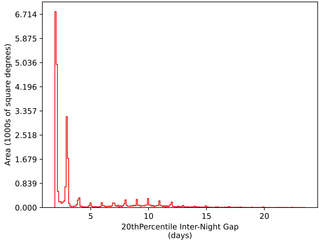
roll_pause_mjdp120_v3.4_10yrs All sky i band: 20thPercentile Inter-Night Gap
