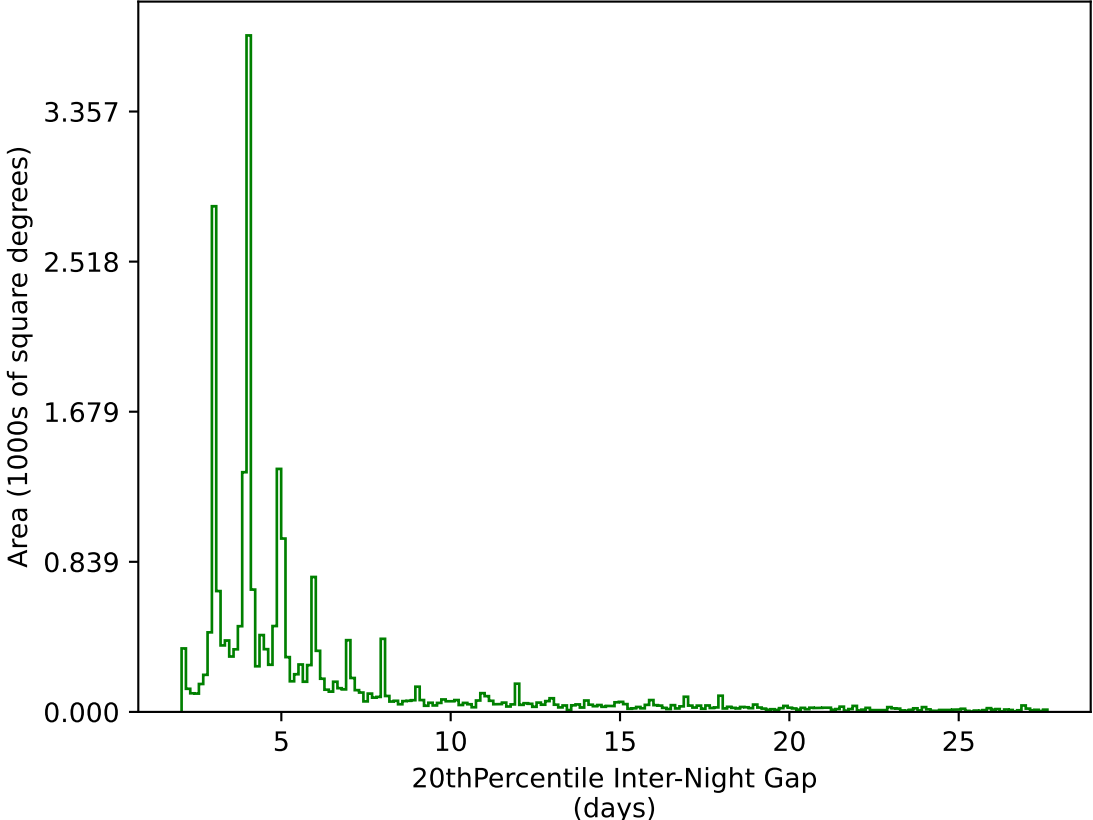
roll_pause_mjdp120_v3.4_10yrs All sky g band: 20thPercentile Inter-Night Gap
